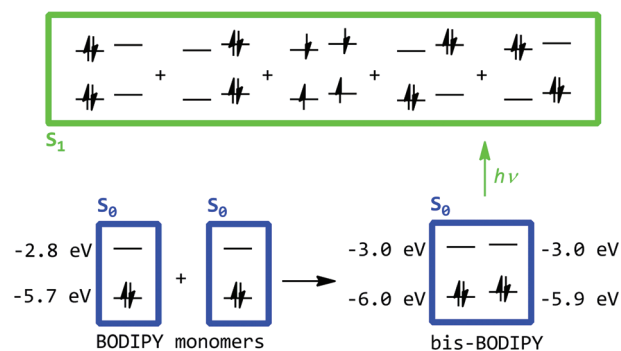
Figure 2. Building up bis-BODIPY S_1 wave function. MO energies are for the 8,8' dimer (3). In the S_1 state, only the leading configurations are shown, and minus signs to restrain antisymmetry are intentionally excluded for clarity.
